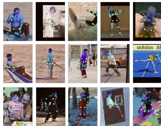
Figure 9. Qualitative results on the MS COCO 2017 validation set produced from HRNet-w32 with our proposed DSRL.
